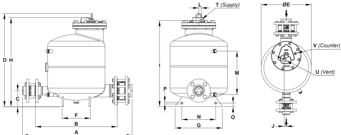
DIMENSIONS (mm)
