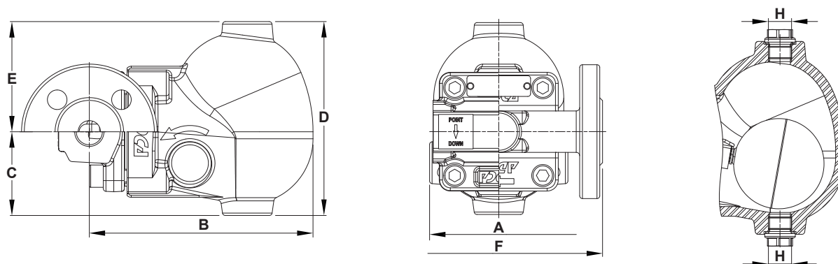
Inline design
